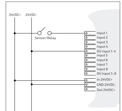
Wiring example with external 24VDC Power supply.
