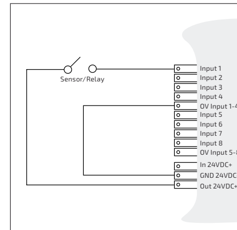
Wiring example with internal 24VDC Power supply.
